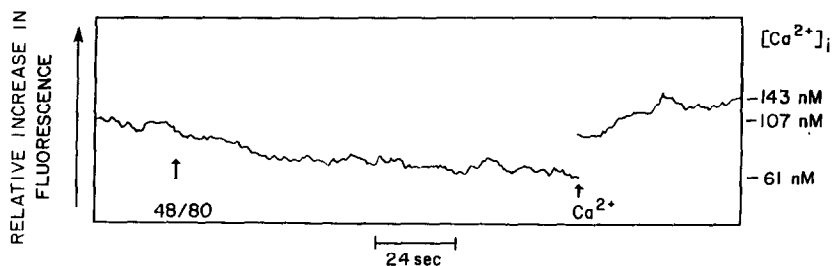
Fig.3. Change in fluorescence from quin 2/AM loaded mast cells bathed in Ca-free Locke following stimulation by compound 48/80 ( 1 \mu\text{g/ml} ), first arrow, and the addition of Ca ( 1 mM), second arrow. A less than 5 s break in the recording occurred when Ca was added.
